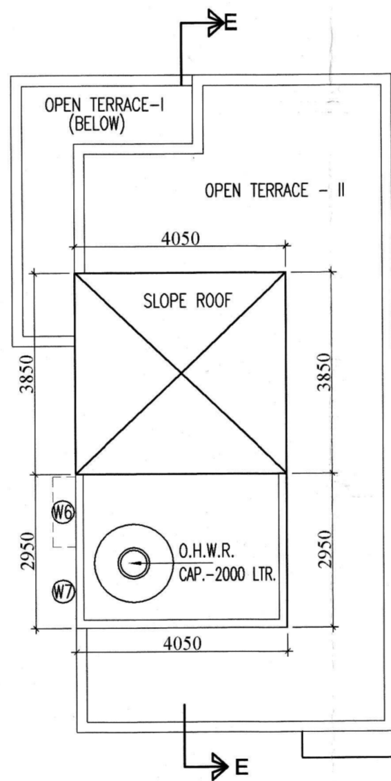
ROOF PLAN
